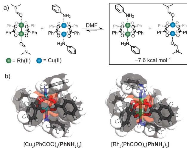
Fig. 5 (a) The ligand exchange reaction between Cu(II) and Rh(II) paddle-wheel complexes as investigated by DFT calculations; (b) a comparison of the optimized structures of [Cu_2(PhCOO)_4(PhNH_2)_2] and [Rh_2(PhCOO)_4(PhNH_2)_2] .
