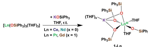
Scheme 2 Synthesis of 1-Ln ( \text{Ln} = \text{Ce},^4 \text{Pr},^4 \text{Nd}, \text{Gd} ).
