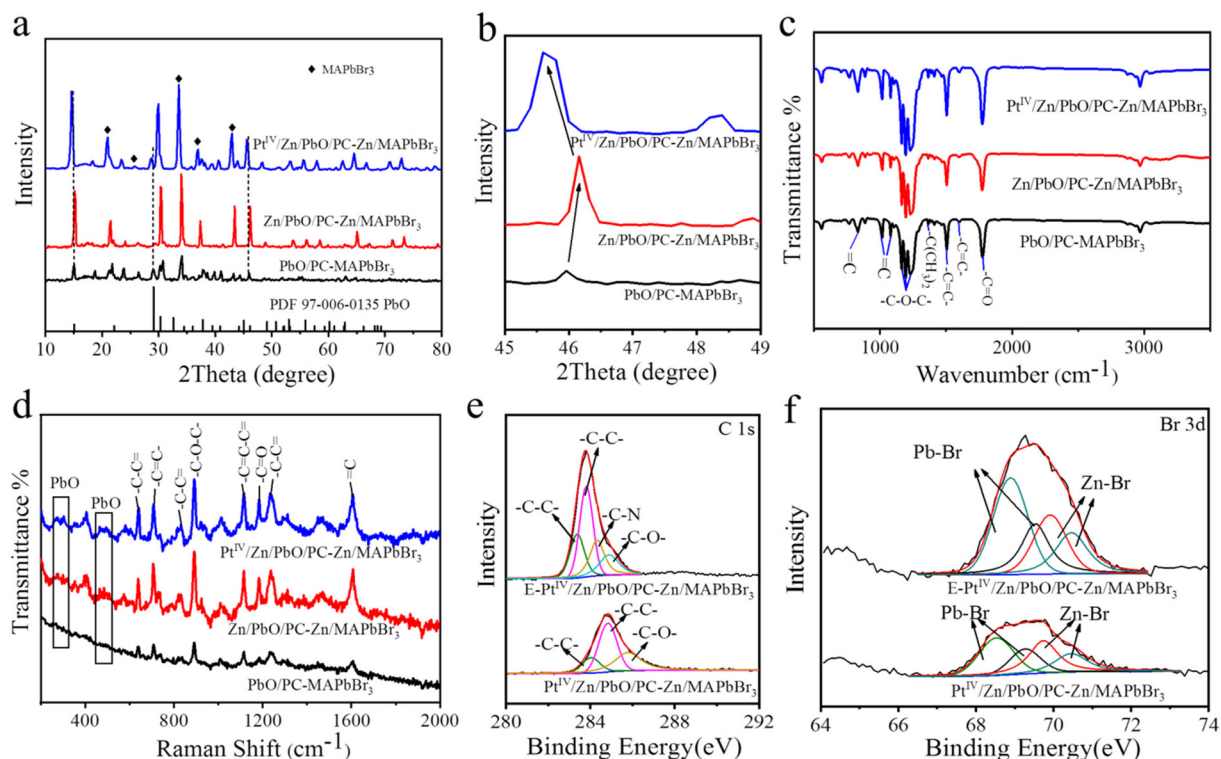
Fig. 2 Chemical characterization of PbO/PC-MAPbBr 3 , Zn/PbO/PC-Zn/MAPbBr 3 and Pt IV /Zn/PbO/PC-Zn/MAPbBr 3 . (a) XRD patterns. Dotted lines are the sectional PbO characteristic patterns. (c) FTIR spectra. (d) Raman spectra. XPS spectra of C 1s (e) and Br 3d (f) for Pt IV /Zn/PbO/PC-Zn/MAPbBr 3 with and without etching.
