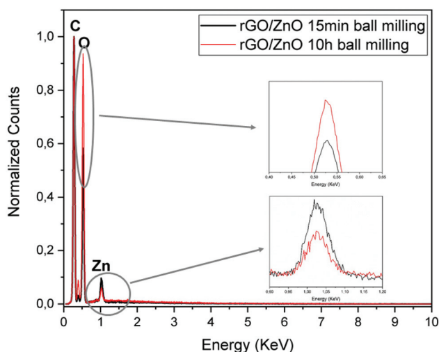
Fig. 5 EDX results of the rGO/ZnO hybrid composite.
