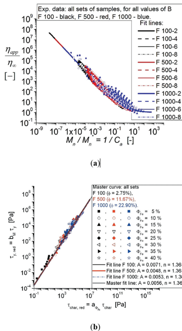
Fig. 38 Ferrofluid based MR fluids. (a) The dependence \eta_{app}/\eta_{\infty} = f(Mn/Mn^* = 1/C_a) for different values of the Fe particle volume fraction \Phi_{Fe} and of the magnetic nanoparticle volume fraction \phi . Fit lines: \eta_{app}/\eta_{\infty} = C_a + 2C_a^{1/2} + 1 . Fit parameter values are given in ref. 696; (b) master curve obtained for all samples with different nano and micro concentrations, at different values of magnetic field induction. a_{\phi} and b_M are horizontal and vertical translation coefficients of experimental data (reproduced from ref. 697 with permission from The Society of Rheology, copyright 2018).
