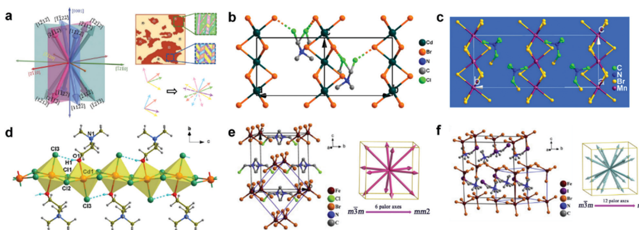
Fig. 5 Different structures of multiaxial ferroelectric halide perovskites. (a) Demonstration of twelve different polarization directions of the TCMC-MnCl 3 perovskite and the corresponding experimental evidence from PFM measurements. Reproduced with permission from ref. 48. Copyright 2017, American Association for the Advancement of Science. (b) Crystal structure of [(\text{CH}_3)_3\text{NCH}_2\text{Cl}]\text{CdBr}_3 in the ferroelectric phase. The dashed lines represent the Cl-Br interactions. Reproduced with permission from ref. 72. Copyright 2018, American Chemical Society. (c) Crystal structure of [(\text{CH}_3)_3\text{NCH}_2\text{X}]\text{MnBr}_3 in the ferroelectric phase. Reproduced with permission from ref. 73. Copyright 2017, American Chemical Society. (d) Crystal structure of [\text{Me}_3\text{NCH}_2\text{CH}_2\text{OH}]\text{CdCl}_3 with the edge-sharing \text{CdCl}_5\text{O} octahedra structure. The cations are coordinated alternatively above and below the perovskite framework. Reproduced with permission from ref. 74. Copyright 2020, American Chemical Society. (e) Crystal structure of (\text{TMCM})\text{FeBr}_4 and the corresponding six equivalent polarization directions. (f) Crystal structure of (\text{TMIM})\text{FeBr}_4 and the corresponding twelve equivalent polarization directions. Reproduced with permission from ref. 75. Copyright 2020, Elsevier.
