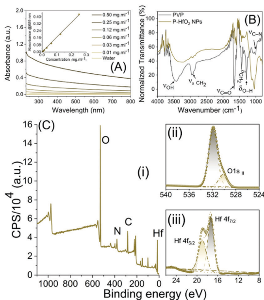
Fig. 3 (A) UV-Vis absorbance spectra of NPs at various concentrations, (B) FTIR spectra; (C) XPS spectra in (i) survey mode, (ii) O1s region and (iii) Hf 4f region.
