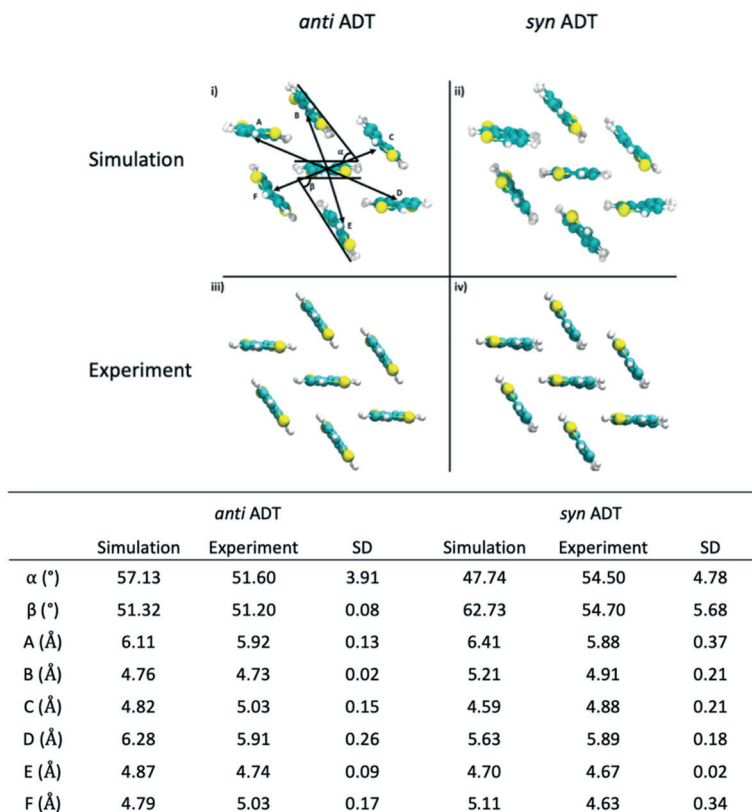
Fig. 8 Comparison of crystalline packing of anti ADT and syn ADT as extracted from a series of snapshots after simulation box crystallization to the experimentally reported crystal structure. Molecular distances and angles are reported in table with standard deviations for each angle and distance.
