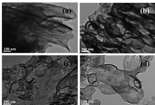
Fig. 15 TEM images of bulk \text{g-C}_3\text{N}_4 (a), alongside porous \text{g-C}_3\text{N}_4 exfoliated at 450^\circ\text{C} (b), 500^\circ\text{C} (c), 550^\circ\text{C} (d). The heat decomposes certain areas of the nanosheets, leaving the resultant sheets ranging from slightly exfoliated and porous to fully exfoliated and with large holes. Reproduced with permission from ref. 188. Copyright 2015 Elsevier B.V.
