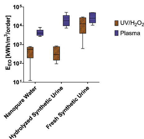
Fig. 4 Calculated electric energy per order ( E_{EO} ) (kW h m -3 per order) for both bench-scale reactors in the nanopure water and synthetic urine matrixes. The box and whisker plot displays 95% confidence intervals for E_{EO} values ( n = 6 , all pharmaceutical compounds in each data point).
