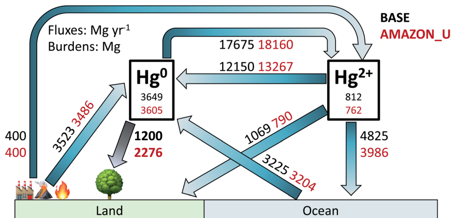
Fig. 6 Atmospheric Hg budget for BASE and AMAZON_U simulations for year 2015. Atmospheric burdens are listed in units Mg and fluxes in Mg per year. The Hg^{2+} burden and fluxes include both gaseous and particulate Hg^{2+} .
