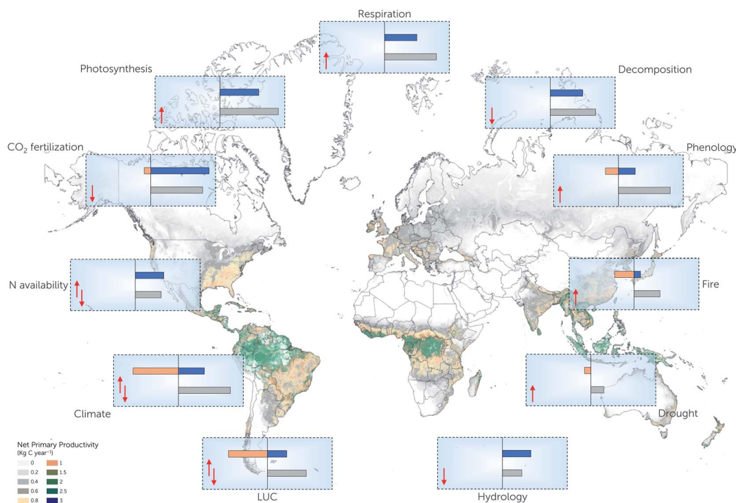
Fig. 2 Schematic of major terrestrial carbon drivers that lead to positive (blue bar) or negative (red bar) feedback loops to the environment. The bar plots signify the simplified form of understanding the feedback in the system. The confidence in the scientific understanding of the system is signified by the grey bar. The upward arrow represents the source and the downward arrow signifies the concurrent sink for predominant carbon pools under changing climate. The superimposed NPP map is for the year 2020, produced from MODIS, https://lpdaac.usgs.gov/products/mod17a3hv006/ .
