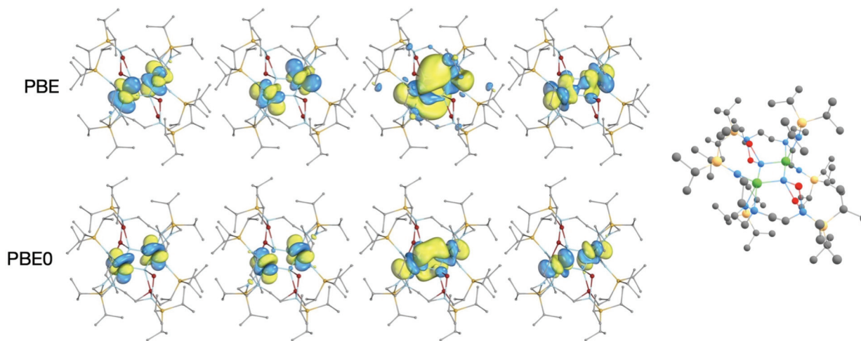
Fig. 4 Singly-occupied \alpha -spin Kohn Sham MOs of the {}^5A_g ground state of 2-opt (top: PBE, bottom PBE0). The isosurfaces enclose 90% of the orbitals. Hydrogen atoms are omitted for clarity. The ball and stick representation of 2-opt is shown to provide orientation of the molecular orbital representations.
