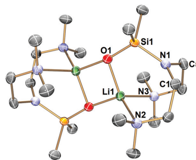
Fig. 5 X-ray crystal structure of [\text{Li}\{\kappa^3\text{-O},N,N'\text{-OSiMe}_2\text{N}(\text{CH}_2\text{CH}_2\text{NMe}_2)_2\}]_2 ( 3 ) at -123 \text{ }^\circ\text{C} with 50% probability ellipsoids. Hydrogen atoms are omitted for clarity. The selected bond distances ( \text{\AA} ) and angles ( ^\circ ) are: Li1–O1 1.851(3); Li1–N2 2.213; Li1–N3 2.232; Si1–O1 1.5794(13); Si1–N1 1.7439(16); N1–C1 1.454(2); N1–C5 1.454(2); Si1–N1–C5 121.65(12); Si1–N1–C1 123.14(12); C1–N1–C5 115.21(15).
