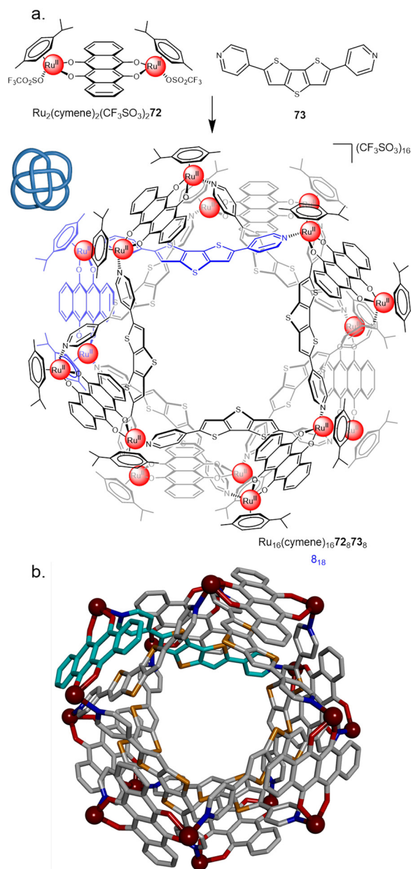
Fig. 25 (a) Synthesis of 8_{18} metalla-knot \text{Ru}_{16}(\text{p-cymene})_{16}\mathbf{72_873_8} . (b) X-ray crystal structure of the 8_{18} metalla-knot with p -cymene ligands omitted for clarity. 100
