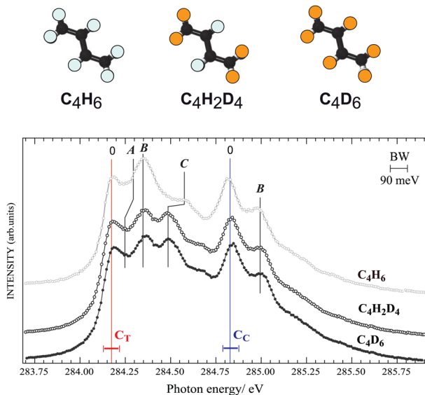
Fig. 2 Ion-yield spectra of normal, partially ( C_4H_2D_4 ) and fully deuterated ( C_4D_6 ) butadiene for C\ 1s-\pi^* excitation. The locations of the deuterium atoms on the isotopes are indicated by orange, and hydrogen atoms by white in the upper panel. The peak positions of resonant features in the terminal ( C_T ) and central ( C_C ) carbons are indicated by the solid vertical lines and labelled as discussed in the text. The photon energy was calibrated using the known argon 2p resonance energies, and the photon bandwidth is 90 meV, also indicated in the figure.
