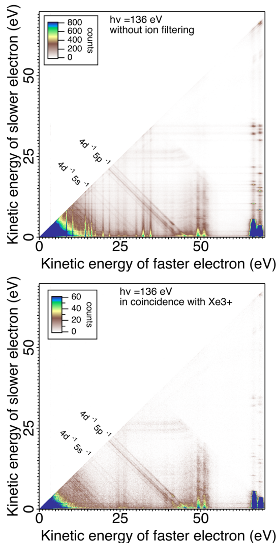
Fig. 5 Coincidence map shows the energy of the slow electron as a function of the kinetic energy of the fast following core valence double photoionization of Xe atoms at 136 eV photon energy. Top: Coincidence map for events where three electrons were detected in coincidence (without ion filtering). Bottom: Coincidence map for events where three electrons were detected in coincidence with \text{Xe}^{3+} .
