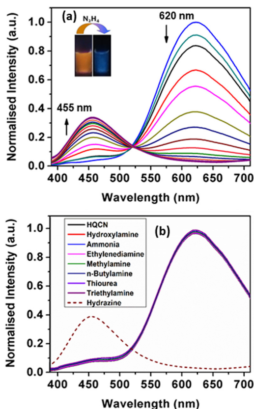
Fig. 3 (a) Fluorescence emission spectra of HQCN ( 10 \mu\text{M} in \text{CH}_3\text{OH}-\text{H}_2\text{O} ; 1/4, v/v in the presence of HEPES buffer (10 mM) solution at pH = 7.2) upon the gradual addition of \text{N}_2\text{H}_4 (0 to 5 equivalents) where the \lambda excitation was 370 nm. Ratiometric spectra of HQCN were observed after the addition of \text{N}_2\text{H}_4 . The emission spectra of HQCN at 620 nm gradually decreased and the peak at 455 nm gradually increased after the addition of hydrazine with an isoemissive point at 520 nm, inset shows the visible emission of HQCN in the absence and presence of 2 equivalents of hydrazine upon irradiation under UV light, (b) Fluorescence emission spectra of HQCN ( 10 \mu\text{M} in \text{CH}_3\text{OH}-\text{H}_2\text{O} ; 1/4, v/v in the presence of HEPES buffer (10 mM) solution at pH = 7.2) after the addition of different guest amines (0 to 5 equivalents). Apart from hydrazine, no significant change was observed for other guest amines.
