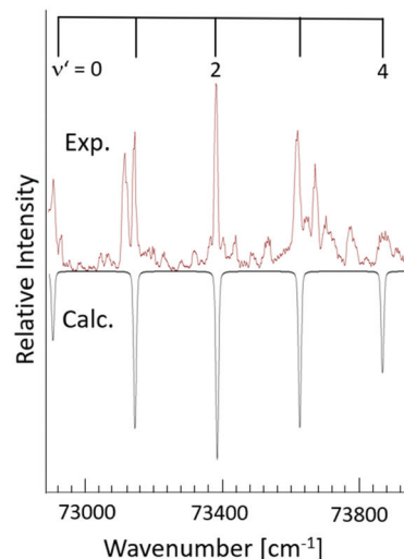
Fig. 3 Vibrational simulation of the transition from the ground state to the 8f\delta_u state. Experimental spectrum on top (red). Calculated spectrum (black, bottom) formed by using a combination of Gaussian line widths of 8 \text{ cm}^{-1} and Lorentzian line widths of 2 \text{ cm}^{-1} (see main text), vibrational temperature of T = 40 \text{ K} , and spectroscopic values of \omega_e = 238 \text{ cm}^{-1} and \omega_e x_e = 0.6 \text{ cm}^{-1} .
