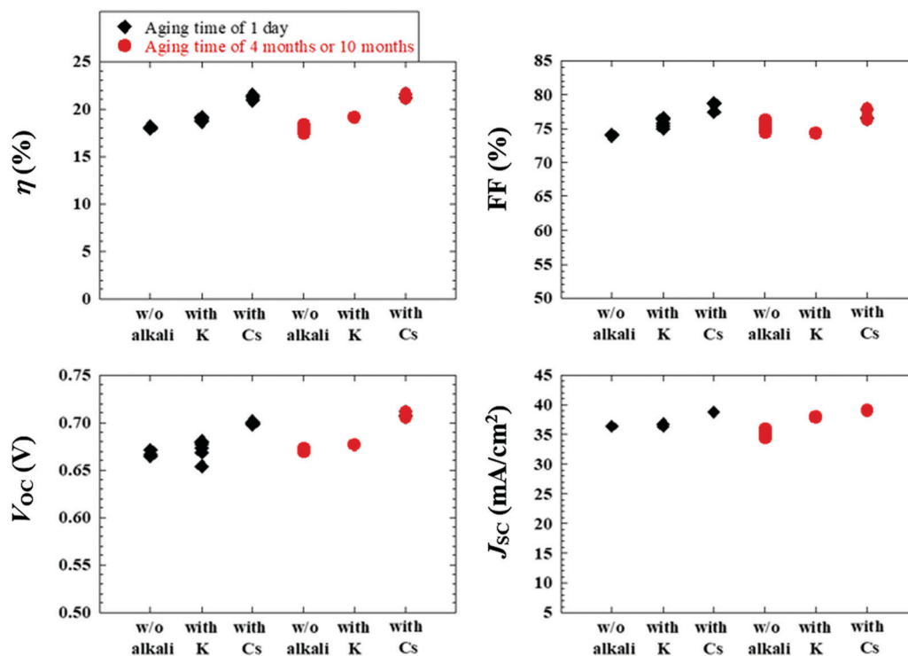
Fig. 17 Photovoltaic performance of the CdS-buffered CIGS 2 solar cells using aged CIGS 2 absorbers for aging times of 1 day, as well as 4 months or 10 months, where the absorbers were processed with and without the alkali (Cs or K) treatment.
