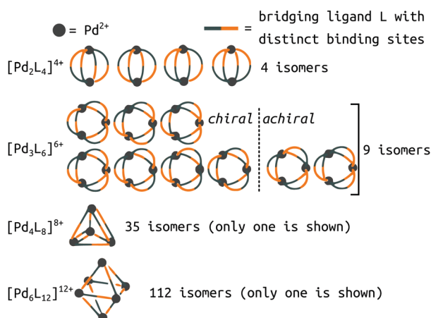
Fig. 8 Potential isomers for metal–ligand assemblies of the general formula [\text{Pd}_n\text{L}_{2n}]^{2n+} ( n = 2, 3, 4 , or 6 ). The isomers differ in the relative orientation of the bridging ligands \text{L} , which have two distinct binding sites. The number of isomers increases from 9 \rightarrow 16 , 35 \rightarrow 68 , and 112 \rightarrow 186 if enantiomers are considered as well. Adapted from ref. 119.
