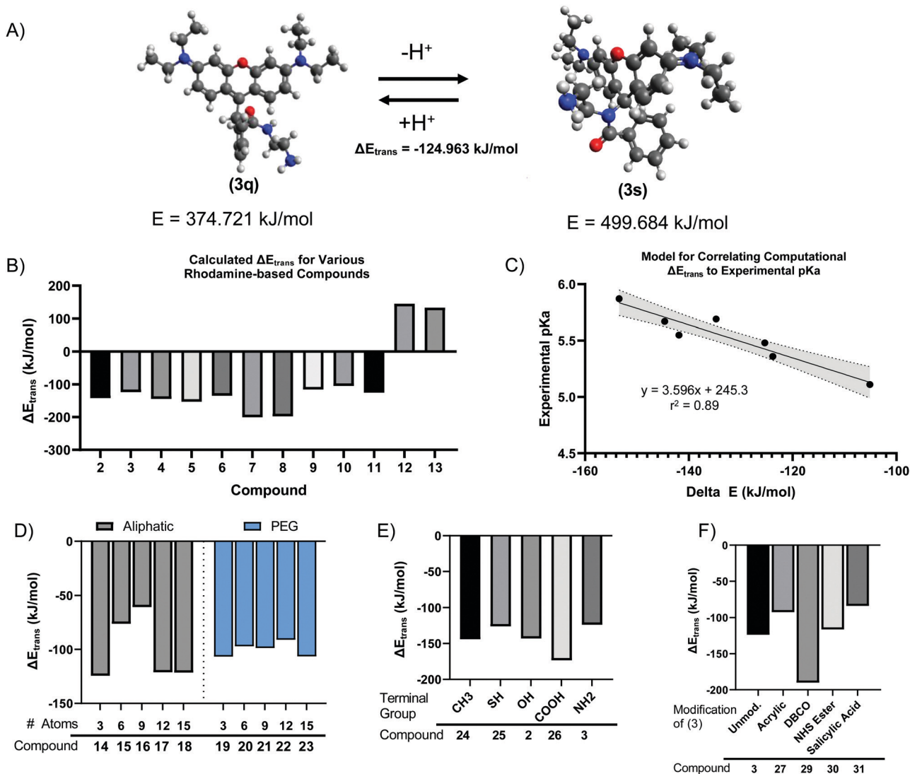
Fig. 3 Ball and stick models of minimum energy geometry-optimized structures of rhodamine 6G ( 1 ) modified by 1,2-ethanolamine ( 3 ) in its quinone (3q) and spirolactam (3s) forms (A). Calculated free energies predict pH-mediated fluorescent properties because of a favorable transition to the quinone state when protonated (B) which correlate with experimental pK_a values (C, shaded area represents 95% confidence interval of the regression). Computational interrogation of theoretical compounds 14–23 to investigate aliphatic chain length-dependence of the energy difference between the spirolactam and quinone forms (D, 14–18 ) and effect of ethylene glycol substitution of the same length (D, 19–23 ). Amide derivatives of ( 1 ) with various terminal functional groups are energetically favorable (E). Amide derivatives, such as ( 3 ), can be further modified favorably to impart specific chemical functionality (F) while maintaining energetically favorable pH-dependent fluorescence.
