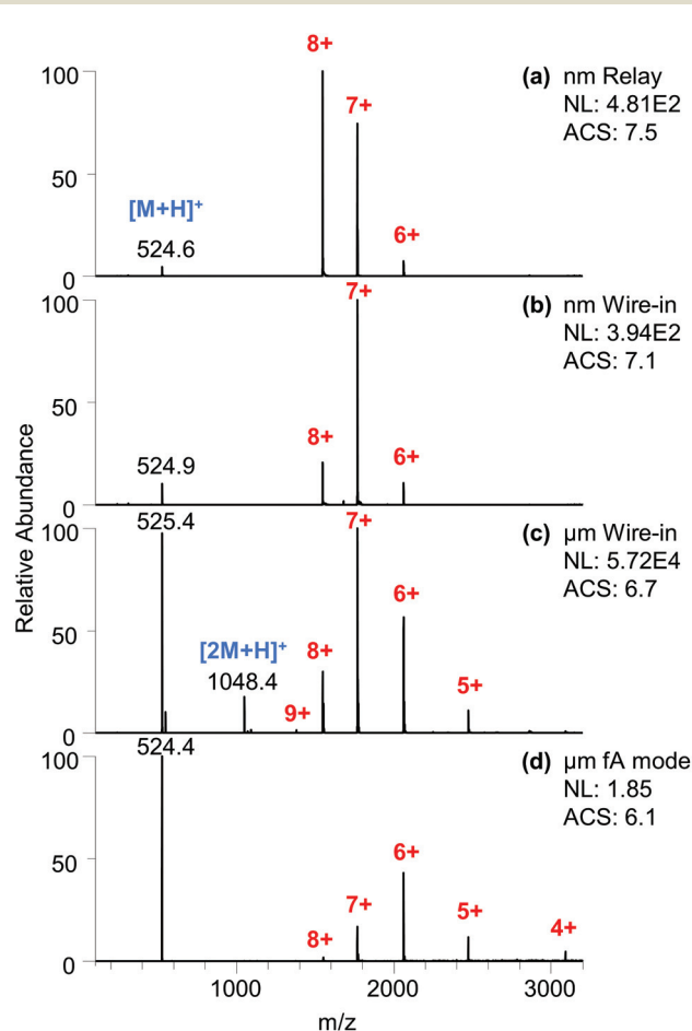
Fig. 3 Full scan mass spectra of a 50 \mu\text{M} cyt c and 50 \mu\text{M} MRFA aqueous mixture under different conditions. (a) Relay ESI using a submicron emitter tip with a 7.7 pL \text{min}^{-1} flow rate. (b) Wire-in ESI using a submicron emitter tip. (c) NanoESI using a micrometer emitter tip. (d) fA ESI using a micrometer emitter tip.
