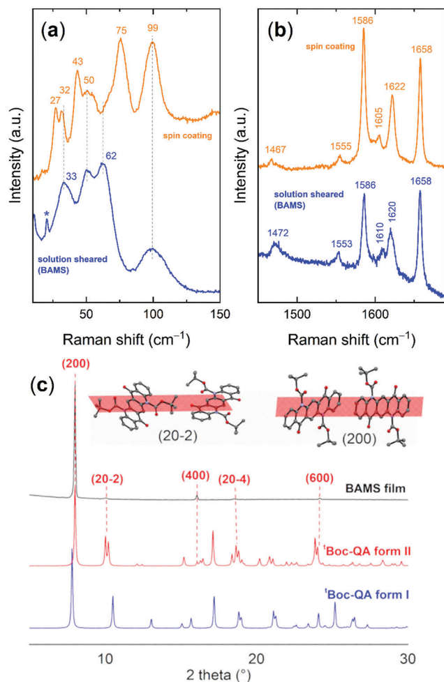
Fig. 6 (a) Lattice phonon and (b) intramolecular Raman spectra of spin cast and BAMS t Boc-QA films; (c) diffraction patterns of BAMS films and the two t Boc-QA polymorphs. Inset: Orientation of the two t Boc-QA molecules with respect of the (20-2) and (200) Miller planes in form II. H CH atoms omitted for clarity.
