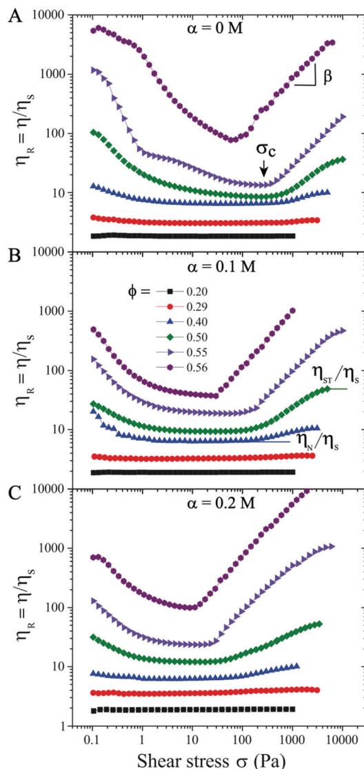
Fig. 1 Rheological flow curves of the relative viscosity \eta_R/\eta_s ( \eta_s being the solvent viscosity) versus the shear stress \sigma for suspensions at different volume fractions ( 0.20 \leq \phi \leq 0.56 ) and salt concentrations ( \alpha ) at (A) 0 M, (B) 0.1 M, and (C) 0.2 M. The pointer in (A) shows the critical stress ( \sigma_c ) for the onset of shear thickening (ST). \eta_N and \eta_{ST} are the plateau viscosities before and after the onset of shear thickening, respectively. In the ST regime ( \sigma > \sigma_c ), \eta \propto \sigma^\beta , where \beta is the ST exponent.
