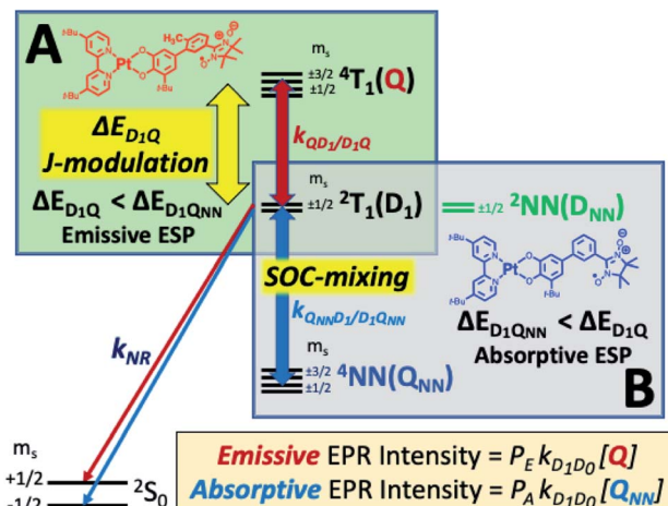
Fig. 5 (A) The reversed quartet mechanism (RQM). Mixing of chromophoric ^2\text{T}_1 and ^4\text{T}_1 states, mediated by conformational J_{\text{SQ-NN}} modulation, gives rise to emissive ESP for 6-Me-mPh-Pt . (B) Spin-orbit induced mixing of chromophoric ^2\text{T}_1 and the NN-based quartet state, ^4\text{NN} , gives rise to absorptive ESP for mPh-Pt . The ^2\text{NN} state can be observed spectroscopically (see ESI†).
