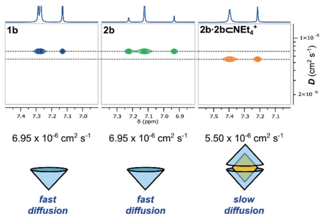
Fig. 4 Truncated ^1\text{H} and DOSY NMR spectra ( d_6 -acetone, 298 K, 500 MHz) of 1b , 2b and 2b \cdot 2b \cdot NEt _4^+ and their diffusion coefficients.
