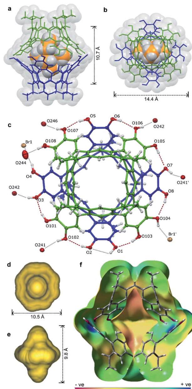
Fig. 5 The X-ray structure of [2a \cdot 2a \cdot NEt _4 ]- Br \cdot 7.63\text{MeOH}\cdot\text{toluene}\cdot 0.37\text{CHCl}_3 with guest, solvent and disorder omitted for clarity where necessary: the host guest complex (a) from the side and (b) top, (c) an ORTEP diagram showing the arrangement of hydrogen-bond donors and acceptors with the NEt _4^+ guest omitted for clarity, the calculated cavity surface (d) shown from the top and (e) side, and (f) a calculated electronic surface potential map of 2' \cdot 2' , showing the electronegative surface of the cavity (see ESI† for details).
