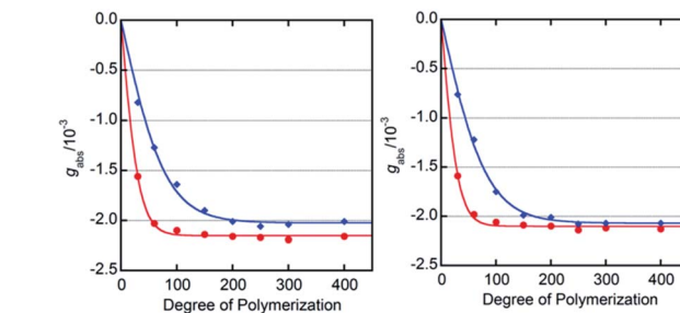
Fig. 3 CD intensities ( g_{\text{abs}} at 367–371 nm at 293 K) of PQX( n ) (ca. 7 \times 10^{-4} M based on monomer units, n = 30, 60, 100, 150, 200, 250, 300 , and 400) in THF ( \blacklozenge ) and MTBE ( \bullet ) in the presence of TFAc-L-Pro-OMe (left) and Ac-L-Pro-OMe (right) (10 mol%).
