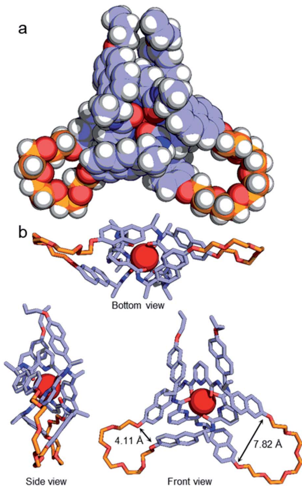
Fig. 3 (a) X-ray crystal structure of \Lambda -4·[Lu], shown in space-filling representation. Selected metal–donor atom bond lengths (Å): Lu–O 2.32(2) × 4, 2.34(2), 2.30; Lu–N 2.46(2), 2.43, 2.44(1). (b) Illustrative stick representations of the crystal structure from several angles. Hydrogen atoms and counteranions omitted for clarity.
