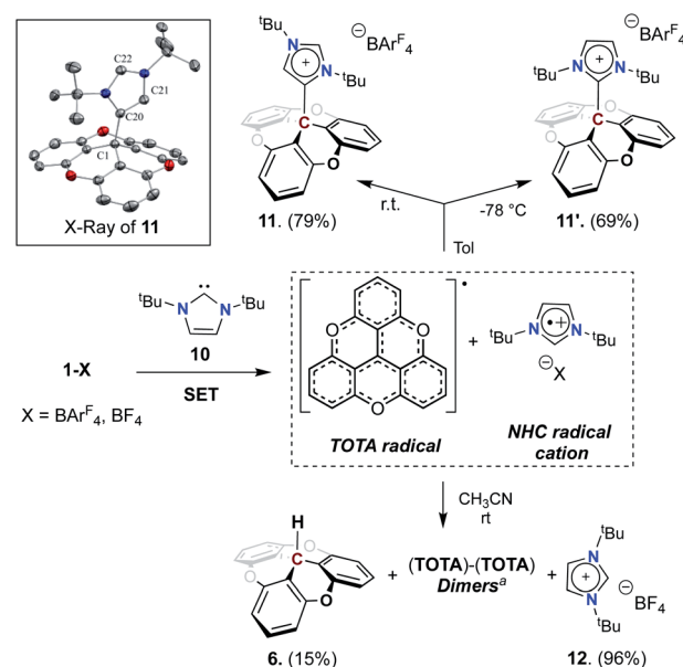
Scheme 4 Reactivity of \text{TOTA}^+ with NHC carbene. a Unless otherwise noted all reactions were carried out on a 0.05 mmol scale using [1]^+ , 0.05 mmol 10 , 4 ml solvent, rt. a See \text{ESI}^\dagger for dimer structures.
