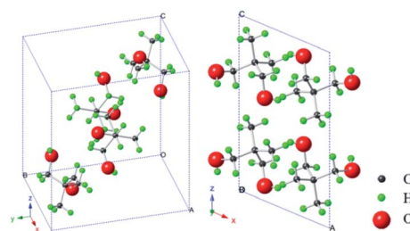
Scheme 1 Crystal structure (monoclinic phase) of NPG at 295 K. 15 Notes: left, view along (1 1 1) crystal plane; right, view along (0 1 0) crystal plane.
