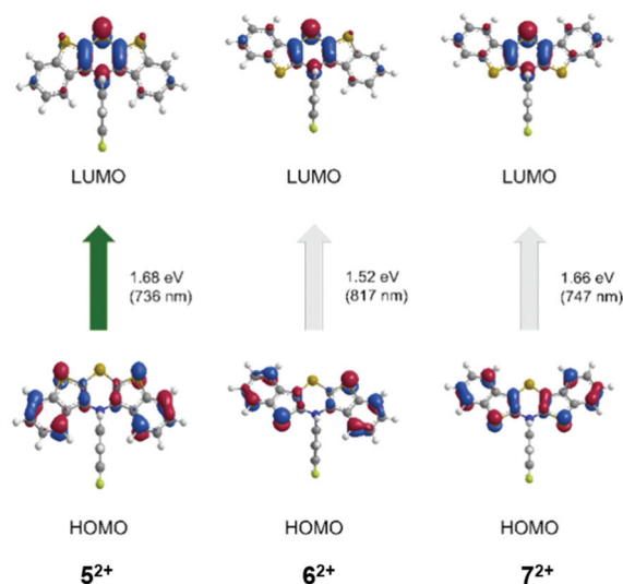
Fig. 12 TDDFT calculated molecular orbital transitions of most bathochromic absorptions of the dicationic species 5 2+ , 6 2+ , and 7 2+ (uB3LYP/6-311++G**, IEFPCM CH 2 Cl 2 , isosurface value 0.05 a.u.) (For further molecular orbital transitions, see ESI†).
