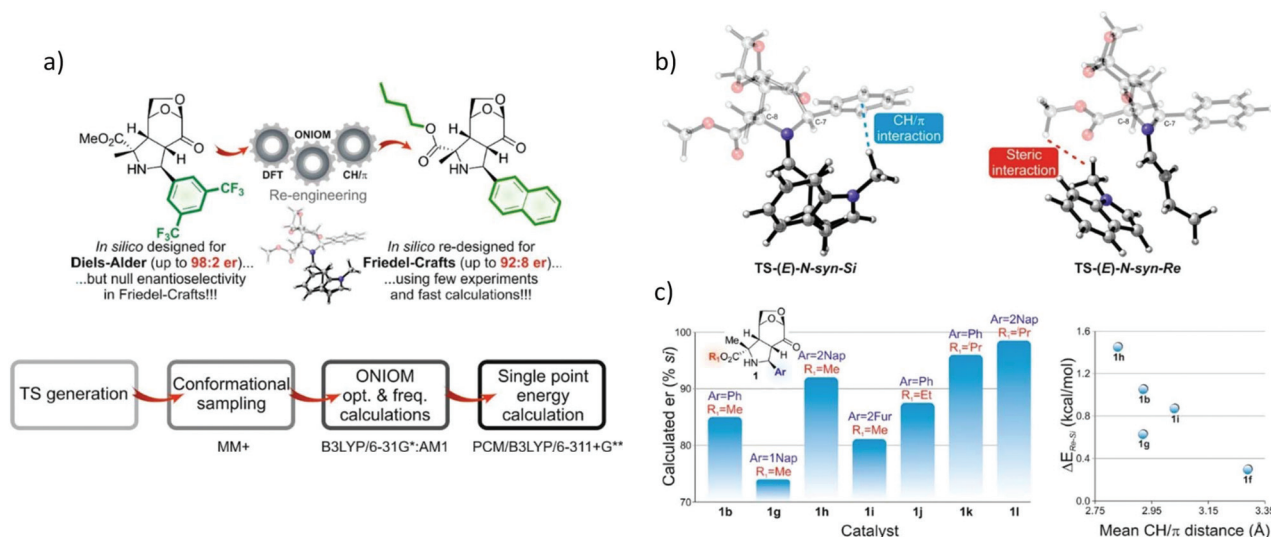
Fig. 14 (a) Catalytic and calculations workflow, (b) the key interactions of Si and Re transition state attack and system partition. The fully-colored image is the high layer and the greyed-out image is the low layer. (c) Predicted enantioselectivity vs. catalyst number (reprint with permission from ref. 93).
