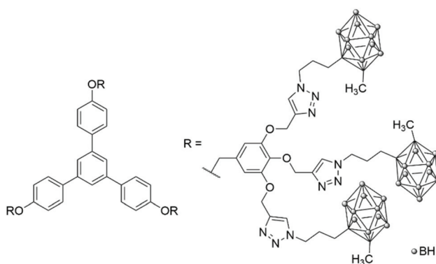
Fig. 9 Phenylene-cored carborane dendrimers prepared by click chemistry.
