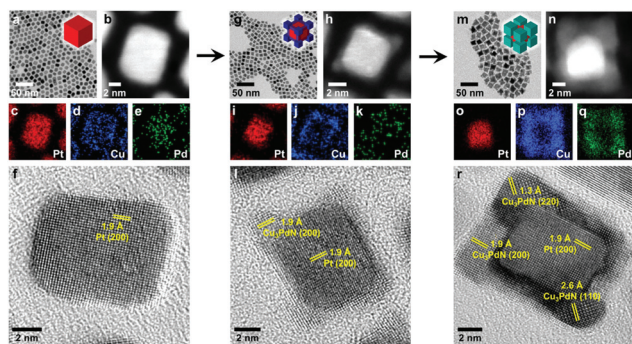
Fig. 13 Time-dependent growth studies of \text{Cu}_3\text{PdN} on Pt nanocubes at 170 °C for (a–f) 5 min, (g–l) 10 min, and (m–r) 15 min. The data for each time point include (a, g, and m) TEM images, (b, h, and n) HAADF-STEM images, (c–e, i–k, and o–q) energy dispersive X-ray spectroscopy (STEM-EDS) element maps for Pt (red), Cu (blue), and Pd (green), and (f, l, and r) HRTEM images of individual particles. Reprinted with permission from ref. 119, Copyright 2019 American Chemical Society.
