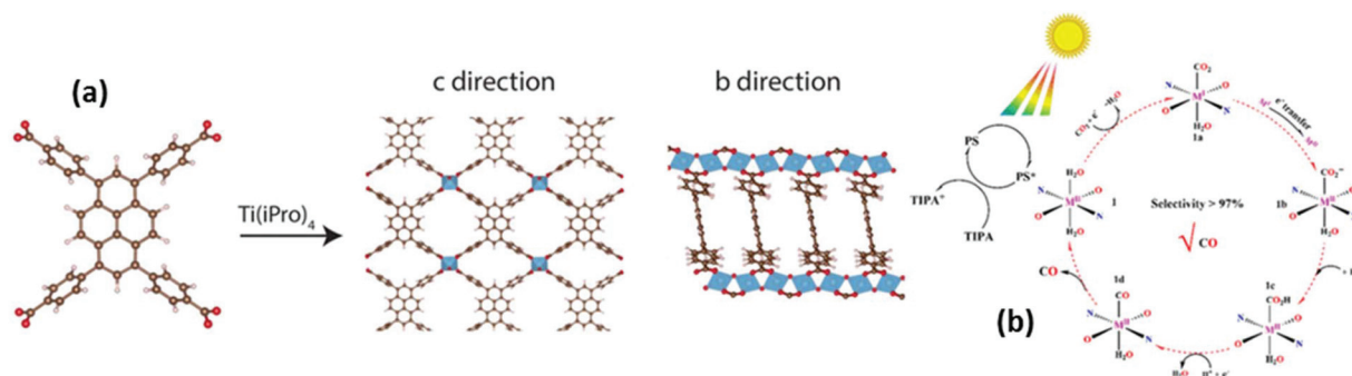
Fig. 7 (a) Schematic illustration of the one-step synthesis of the titanium-based MOF from the 4,4',4''-(pyrene-1,3,6,8-tetrayl)tetrabzoic acid ligand. In the c direction there are views of the stimulated structure emphasizing on the microporous channels, while in the b direction the views of the Ti–O–Ti chains along the b axis are presented. Ti is illustrated with blue colour, C with dark brown and O with red. H atoms are excluded. (a) This figure has been reproduced from ref. 133 with permission from John Wiley and Sons, copyright 2020. (b) Proposed photocatalytic mechanism of MOFs in the presence of PS for the CO 2 photoreduction to CO. (b) This figure has been reproduced from ref. 135 with permission from American Chemical society, copyright 2019.
