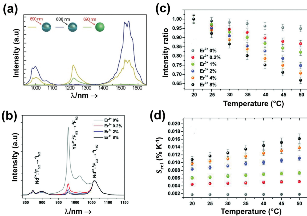
Fig. 28 (a) Room temperature emission spectra of simple core Er 3+ ,Tm 3+ , Yb 3+ :LaF 3 under 690 nm excitation (green) and of active core@active shell Er 3+ ,Yb 3+ :LaF 3 @Er 3+ ,Tm 3+ :LaF 3 (concentrations of lanthanide ions Tm 3+ ,Yb 3+ and Er 3+ are 10 mol%, 10 mol% and 2 mol%, respectively) under 690 (yellow) and 808 nm (blue) laser excitation. The green sphere and the grey core covered with a blue sphere represent the simple core and the active core@active shell, respectively. Reprinted with permission from ref. 240. Copyright 2017, Wiley-VCH Verlag GmbH & Co. KGaA. Effect of the Er 3+ concentration on: (b) the intensity of the emissions, (c) the intensity ratio, and (d) S rel on Tm 3+ ,Yb 3+ :SrF 2 @Y 3+ :SrF 2 @Er 3+ ,Nd 3+ ,Yb 3+ :SrF 2 @Nd 3+ :SrF 2 nanocrystals. (b)–(d) Adapted with permission from ref. 242. Copyright 2018, The Royal Society of Chemistry.
