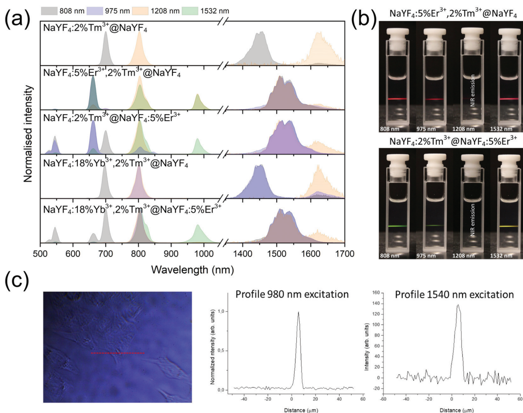
Fig. 8 (a) Comparison of core@shell NPs emission spectra under 808, 975, 1208, or 1532 nm excitation, normalised to the most intense band. (b) Emission of \text{NaYF}_4\text{:}5\%\text{Er}^{3+}, 2\%\text{Tm}^{3+} @ \text{NaYF}_4 and \text{NaYF}_4\text{:}2\%\text{Tm}^{3+} @ \text{NaYF}_4\text{:}5\%\text{Er}^{3+} NPs under various excitations in the form of hexane colloids (1 mg \text{cm}^{-3} ). (c) Confocal microscopy scans under two different excitation wavelengths with cells incubated with \text{NaYF}_4\text{:}5\%\text{Er}^{3+}, 2\%\text{Tm}^{3+} @ \text{NaYF}_4 NPs.
