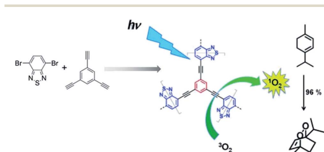
Fig. 2 Synthesis of benzothiadiazole functionalized CMPs. Reproduced with permission. 94 Copyright 2013, John Wiley and Sons.
