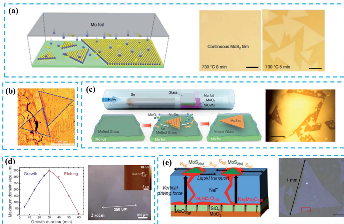
Fig. 3 (a) Schematic diagram of a plane source supply system and typical optical images of \text{MoS}_2 films grown on soda-lime glass by low pressure CVD (LPCVD), scale bar: 200\ \mu\text{m} . Adapted with permission from ref. 45, copyright 2018 Nature. (b) Optical image of millimeter-size triangular monolayer \text{WS}_2 single-crystalline domains on Au foil, scale bar: 500\ \mu\text{m} . Adapted with permission from ref. 46, copyright 2017 Nature. (c) Schematic diagram (left) and optical images (right) of CVD growth of \text{MoSe}_2 crystals on molten glass, scale bar: 500\ \mu\text{m} . Adapted with permission from ref. 13, copyright 2017, American Chemical Society. (d) Evolution of the size of single-crystal \text{MoS}_2 domains as a function of the growth duration (left); optical images of \text{MoS}_2 (right) grown on sapphire after 30 min with \text{O}_2 flow of 2 sccm by LPCVD, scale bar: 100\ \mu\text{m} . Adapted with permission from ref. 38, copyright 2015 American Chemical Society. (e) Schematic diagrams of the growth mechanism (left) of the self-capping vapor-liquid-solid (SCVLS) method (right) and 1 mm \text{MoS}_2 flake grown through the SCVLS method. Scale bar: 200\ \mu\text{m} . Adapted with permission from ref. 32, copyright 2020 Nature.
