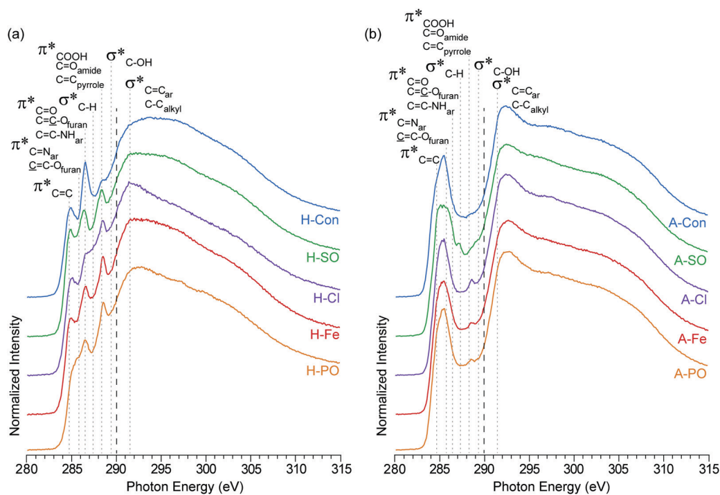
Fig. 3 NEXAFS carbon K-edge spectra of (a) hydrothermal carbons (H-) and (b) activated hydrothermal carbons (A-). Functional group locations for the main \text{C}1\text{s} \rightarrow \pi^* and \text{C}1\text{s} \rightarrow \sigma^* are added for reference and based on previous NEXAFS work on hydrothermal carbons. 17 The long dashed lines represent the position of the arctangent step function at 290.0 eV.
