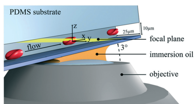
Fig. 5 Sketch of a microfluidic confocal imaging approach. The setup consists of a microchannel with a tilt angle of approximately 3^\circ with respect to the focal plane (yellow) and a spinning microlens enhanced Nipkow disk for confocal cross-sectional imaging. Reproduced from ref. 47 with permission from Appl. Phys. Lett.
