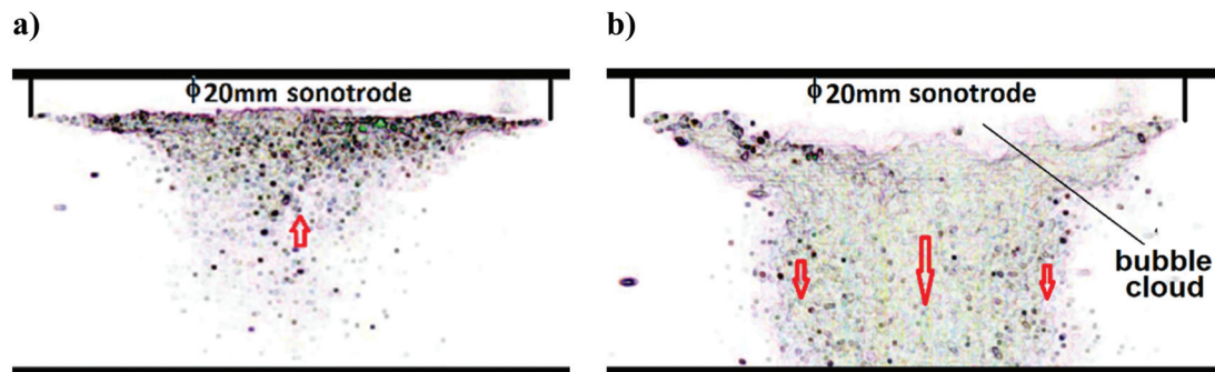
Fig. 1 High speed camera (20k frames per s) snap shot of cavitation underneath a 20 mm diameter sonotrode at: (a) 20 W\ cm^{-2} and (b) 200 W\ cm^{-2} . The direction of bubble movement is indicated by the arrows. The bubbles close to the axis centre line of the sonotrode cylinder are faster than those away from the centre line.
