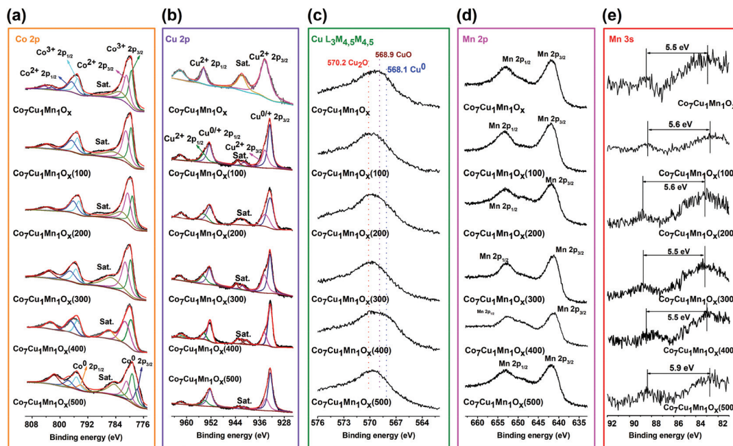
Fig. 3 XPS spectra of the unreduced \text{Co}_7\text{Cu}_1\text{Mn}_1\text{O}_x catalyst and the \text{Co}_7\text{Cu}_1\text{Mn}_1\text{O}_x(100, 200, 300, \text{ and } 500) catalysts, respectively. (a) Co 2p XPS, (b) Cu 2p XPS, (c) Cu \text{L}_{3}\text{M}_{4,5}\text{M}_{4,5} AES spectra, (d) Mn 2p XPS, and (e) Mn 3s XPS, respectively.
