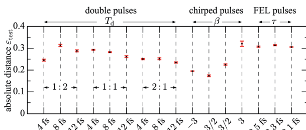
Fig. 2 Absolute distance error \epsilon_{\text{test}} eqn (8d), of the different predicted spectra for test data: double pulses with time delay T_d and amplitude ratios A_1 : A_2 as indicated, chirped pulses with chirp parameter \beta , and partially coherent pulses with coherence time \tau .
