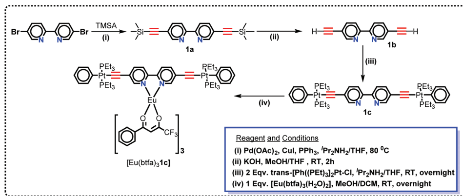
Scheme 1 Synthetic protocol for the Pt(II) di-yne organometallic chromophore and the heterotrimeric (d-f-d) complex.
