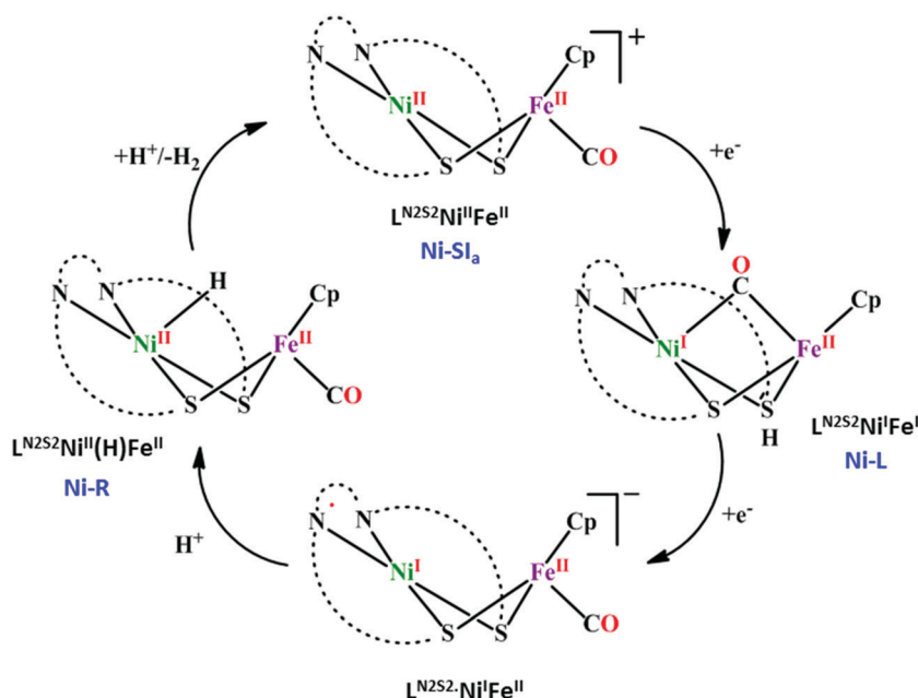
Scheme 32 Proposed mechanistic cycle of proton reduction in complex [\text{L}^{\text{N}2\text{S}2}\text{Ni}^{\text{II}}\text{Fe}^{\text{II}}\text{cp}(\text{CO})]^+ (Fig. 32b).
