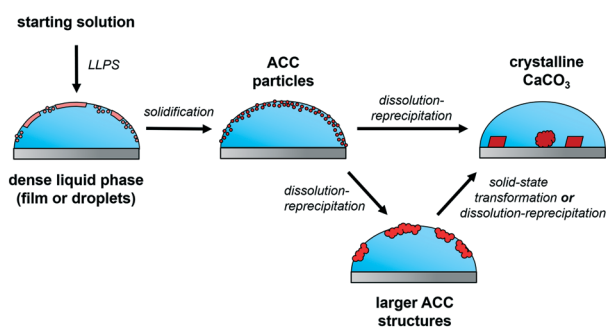
Fig. 4 The proposed mechanism of CaCO 3 crystallization in diffusion-based experiments. The first phase separation in the system is LLPS forming a dense liquid mineral phase. This phase can appear as a film or droplets, depending on the experimental conditions. The liquid precursor phase then solidifies to ACC particles, which in turn dissolve to form larger amorphous structures or directly the crystalline polymorphs. In parallel with the processes shown, ACC particles could form in the solution or crystalline calcium carbonates on the surface of the wafer can occur (not shown in the scheme). Solid-state transformations were also observed for the dried ACC precipitates (Fig. S12†).
