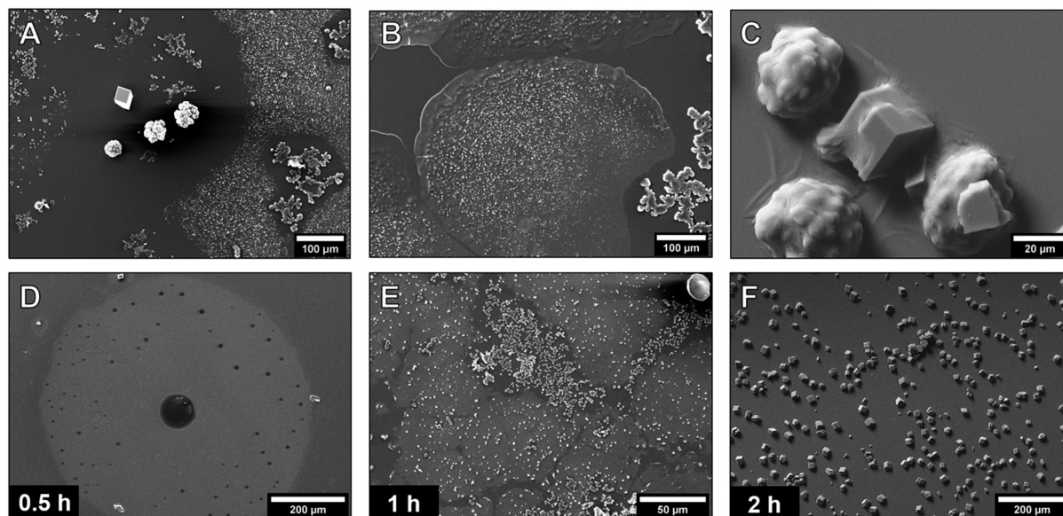
Fig. 3 SEM images for 1 h additive-free gas diffusion experiments using A) 10 mM, B) 20 mM and C) 40 mM CaCl 2 . A) Different structures are visible on the wafer. No films or smaller particles are visible around larger amorphous or crystalline structures, therefore, likely a dissolution–reprecipitation mechanism occurs. B) In many areas of the wafer, large films with smooth edges were detected. Closer to the center of the spherical structures, smaller particles are visible. C) Calcite and vaterite particles are covered by the film. D)–F) Time-dependent development of the precursor films in the additive-free experiments using 10 mM CaCl 2 .
