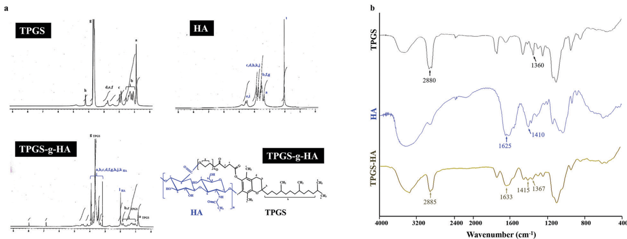
Fig. 2 (a) Nuclear magnetic resonance spectroscopy analyses of (a) TPGS, HA, and TPGS- g -HA; (b) Fourier transform infrared analyses of TPGS, HA, and TPGS- g -HA.
