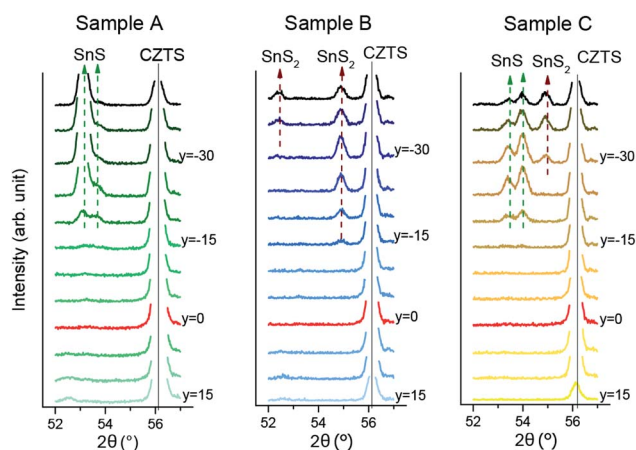
Fig. 4 XRD patterns of samples A, B and C in a 2θ range with expected SnS and SnS 2 reflections. y denotes the distance to the Cu/Sn = 2 line in mm.
